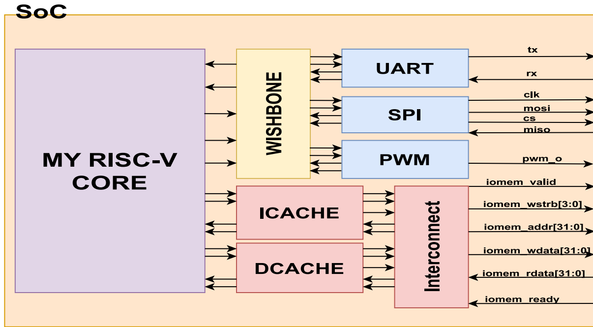
Fig. 2. General structure of the designed processor.
