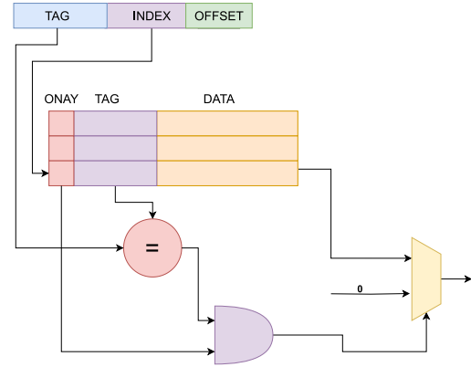
Fig. 8. Direct mapped cache structure.
