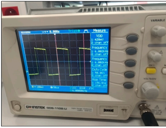
(a) 50% Duty Cycle PWM signal.
