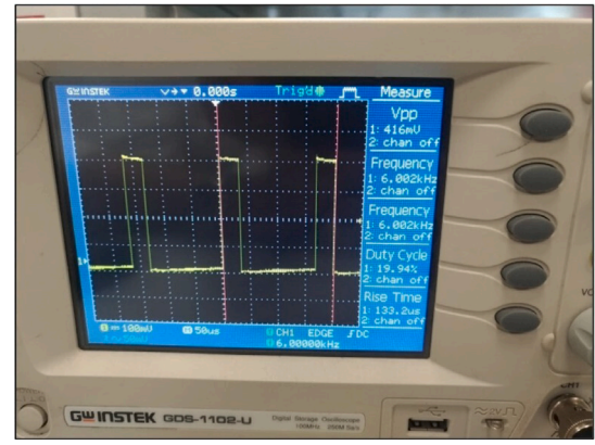
(b) 20% Duty Cycle PWM signal.
