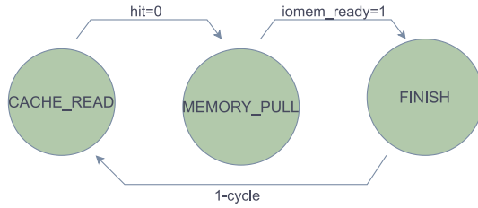
Fig. 9. ICACHE finite state machine structure.
