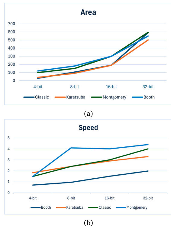
Fig. 1. Illustrates the area occupied by multiplication algorithms and their respective speeds [6].
