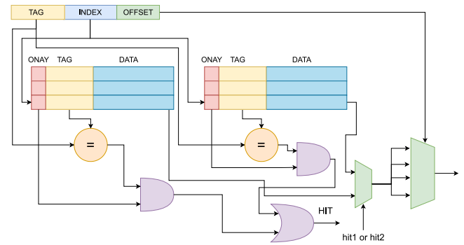
Fig. 10. Structure of DCACHE.
