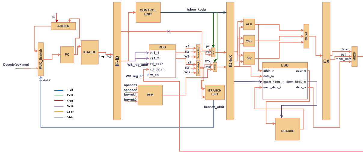
Fig. 3. Data path of designed core.
