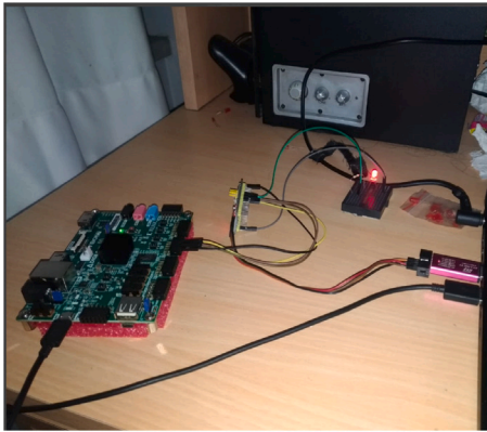
Fig. 18. SPI test with Zybo Z7-20.
