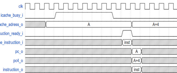
Fig. 4. FETCH phase signal representation.
