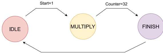
Fig. 6. Finite state machine diagram of multiplication algorithm.
