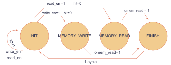
Fig. 11. DCACHE's Finite State Machine Structure.
