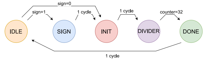
Fig. 7. Finite state machine diagram of division operation.
